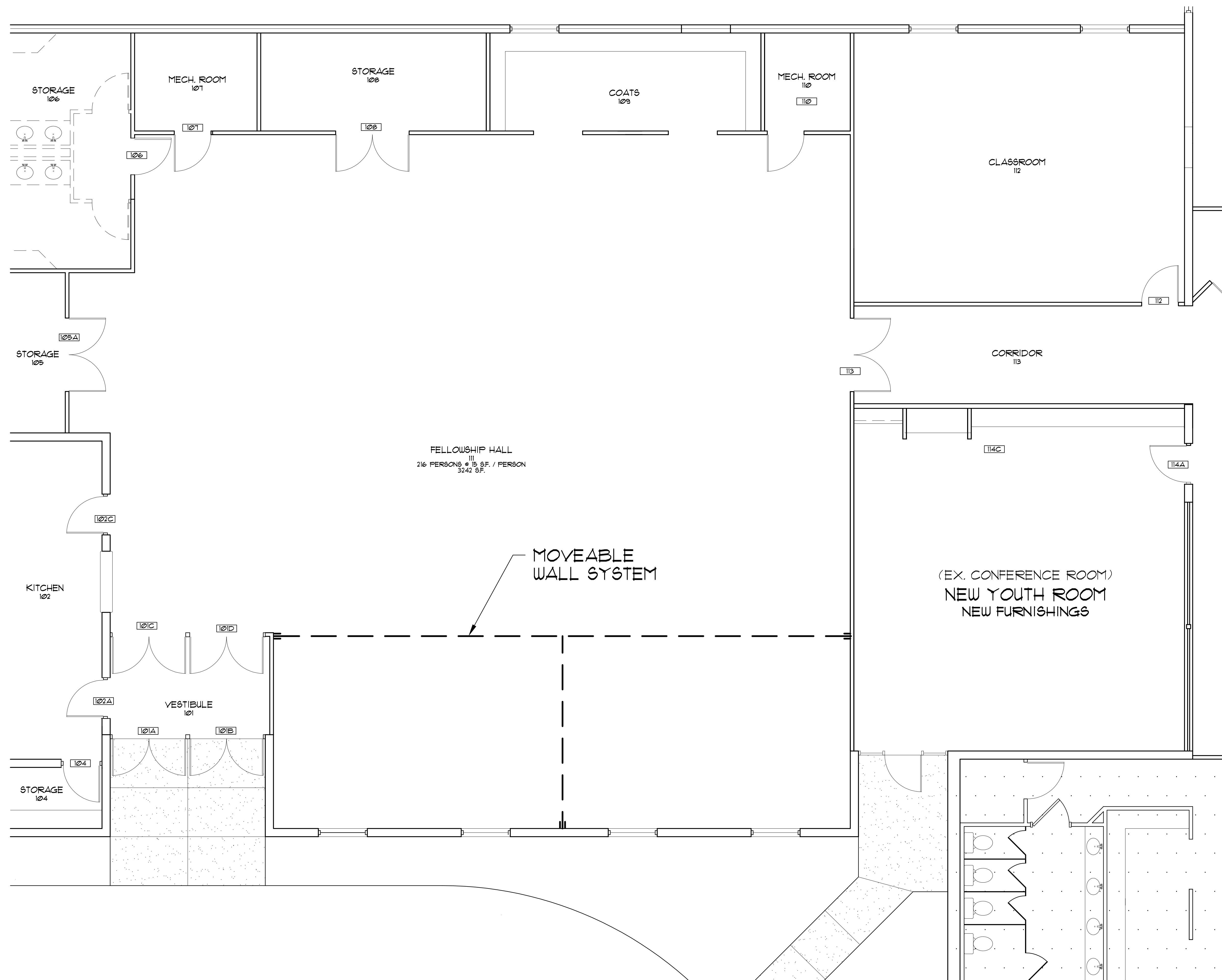
FLOOR PLAN SCALE 1/4" = 1'-0" 03/11/06
